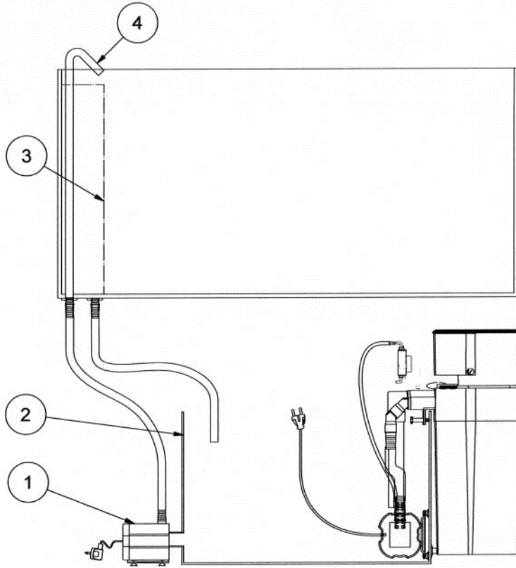
Fig. 5: EVO 1000 set-up next to the filter tank
