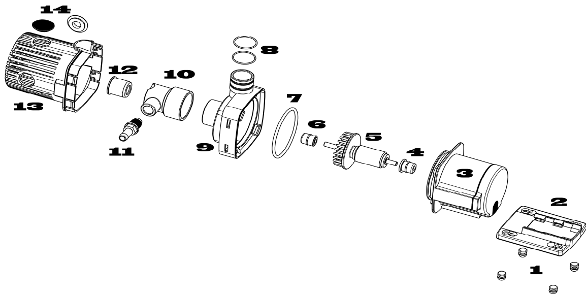
Fig. 2: Venturi pump DC Runner 1.2 incl. 3D-needle wheel
